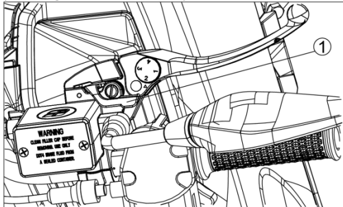
① Hydraulic parking brake lever
